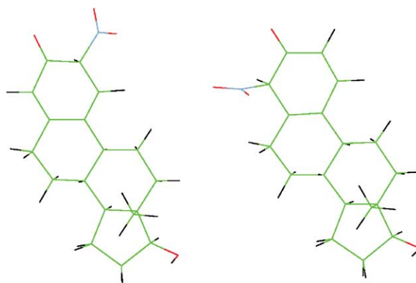
Figure 6. Energy minimized structures of nitroketones formed by coupling of estradiol phenoxyl radical with \text{NO}_2 at C-2 and C-4 position. 32
