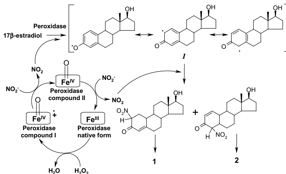
Scheme 1. Proposed mechanism of formation of nitroestradiols 1 and 2 by the peroxidase/ \text{H}_2\text{O}_2/\text{NO}_2^- system.
