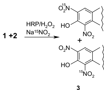
Scheme 2. Formation of 15 N labeled 3 by reaction of 1 and 2 with peroxidase/H 2 O 2 in the presence of 15 NO 2 − .
